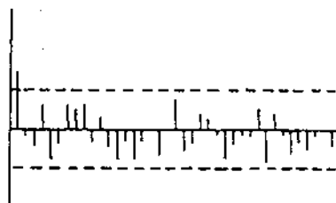
Partial autocorrelation of \nabla \text{Ln} V1
