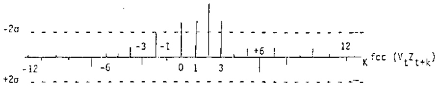
GRAPH 6 CROSS CORRELATION FUNCTIONS (1873 - 1890)
