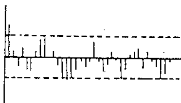
autocorrelation function of \nabla \text{Ln} V1
